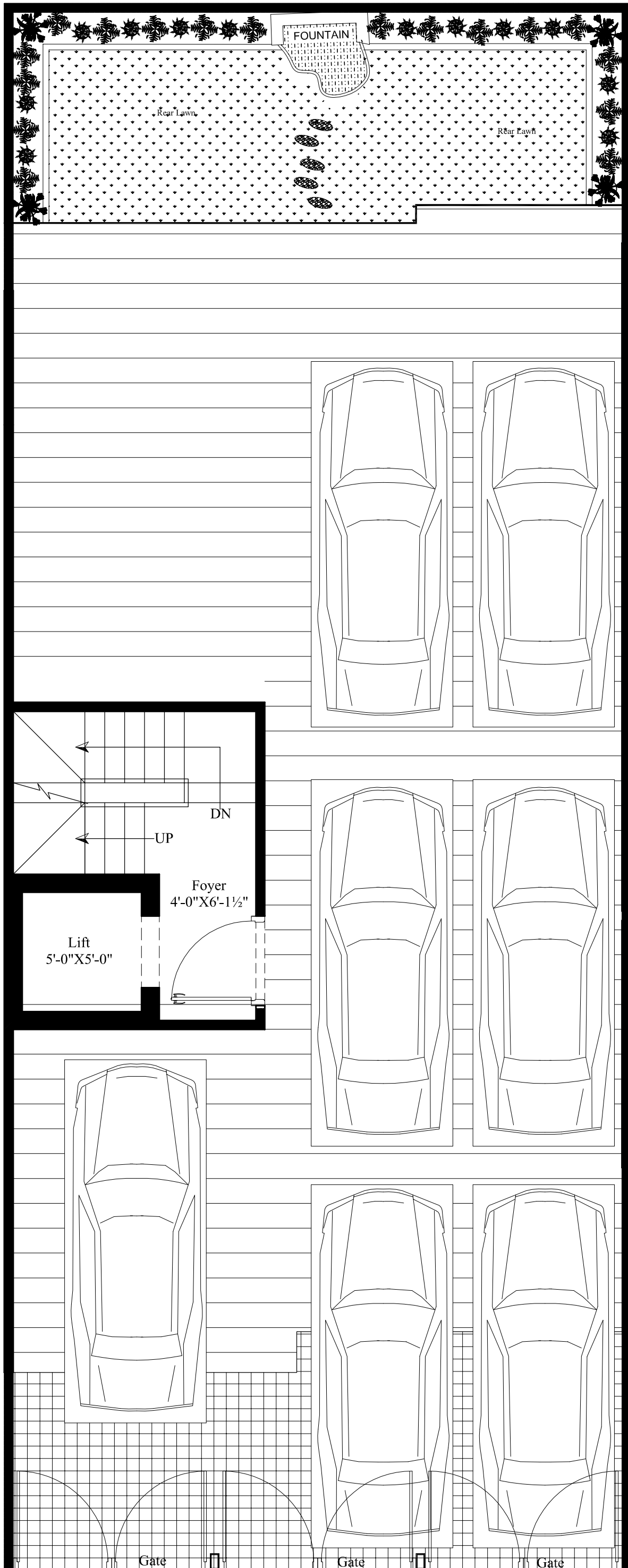
STILT GROUND FLOOR PLAN
