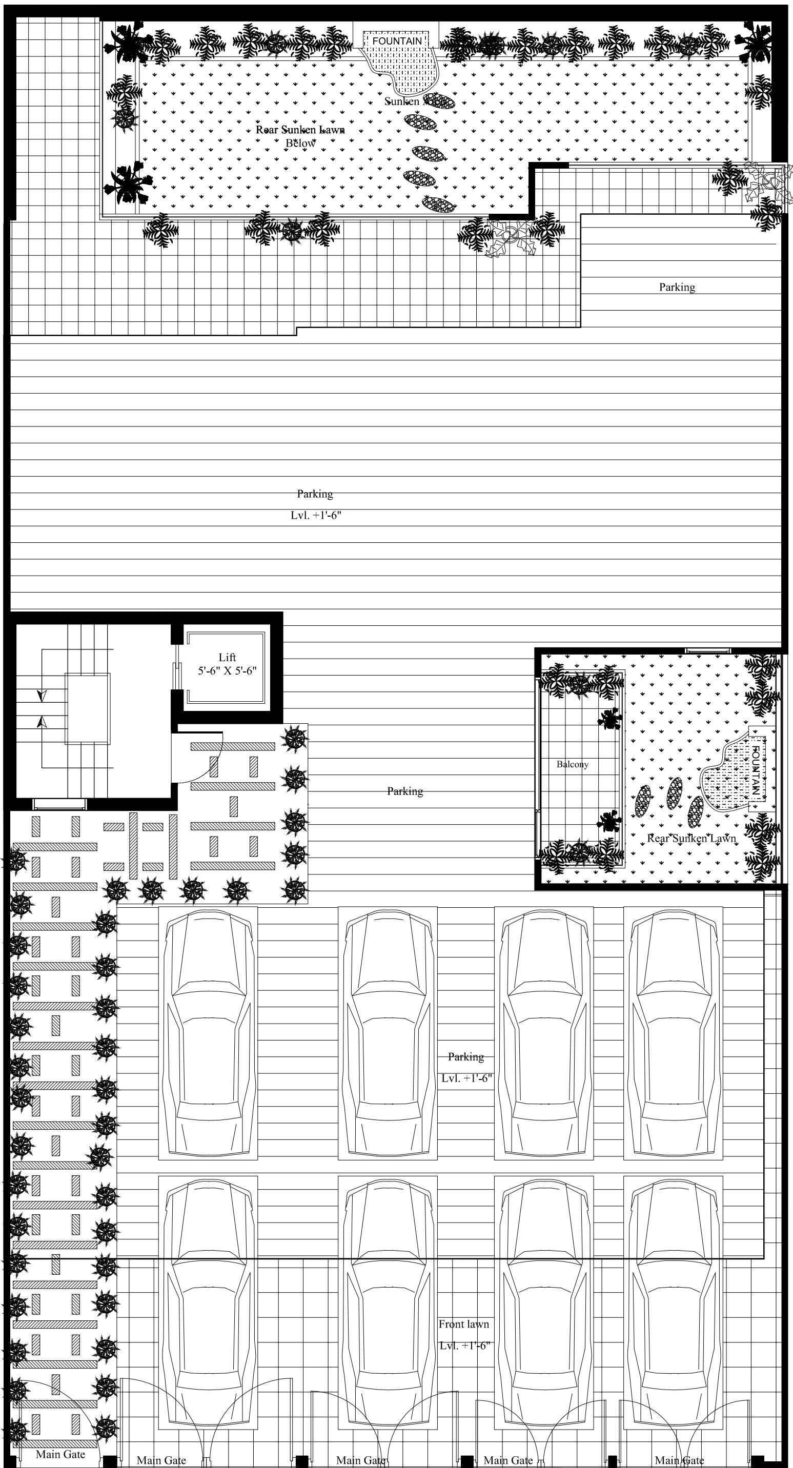
Stilt/ Ground Floor Plan
