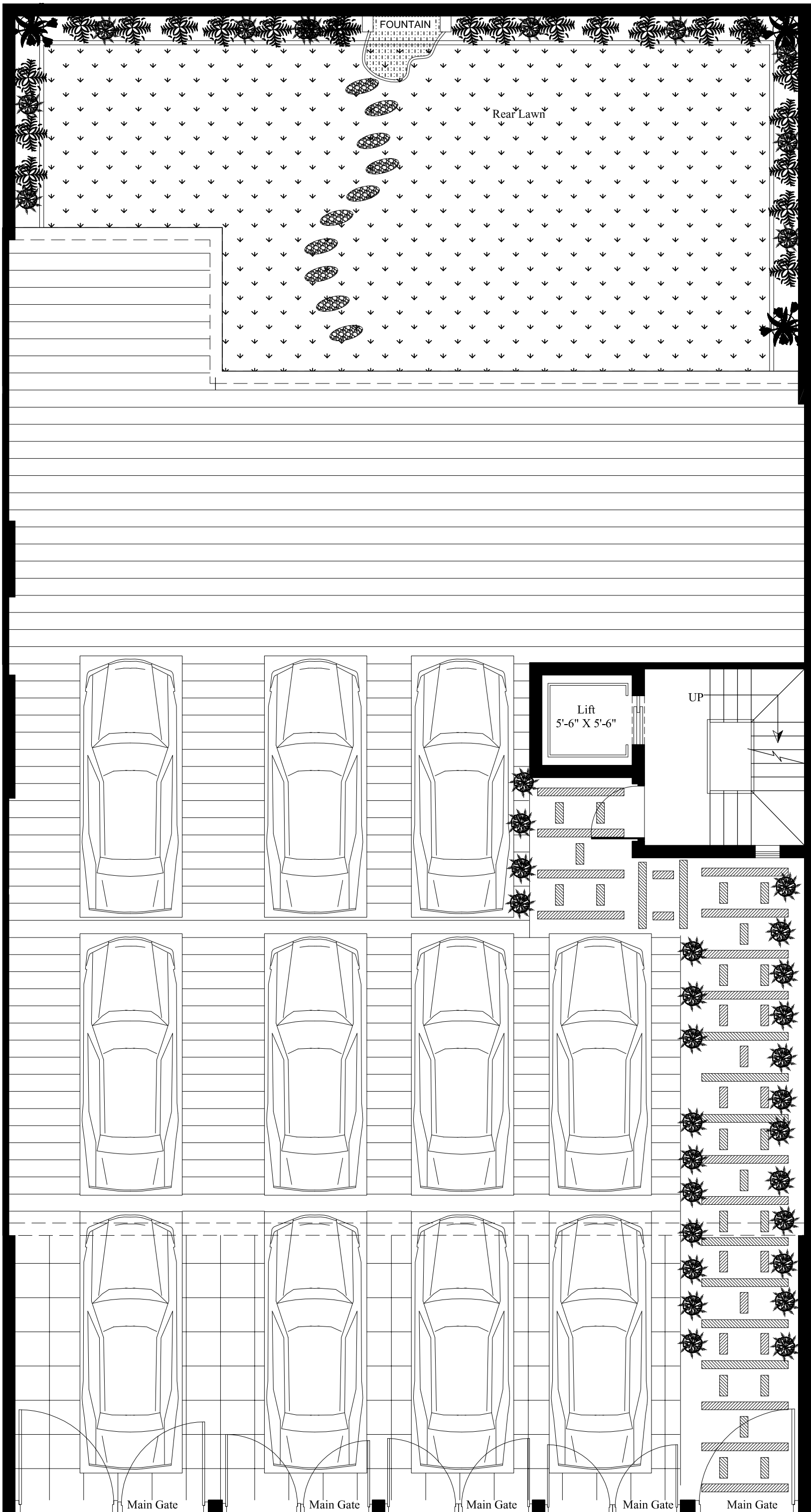
Stilt Ground Floor Plan
